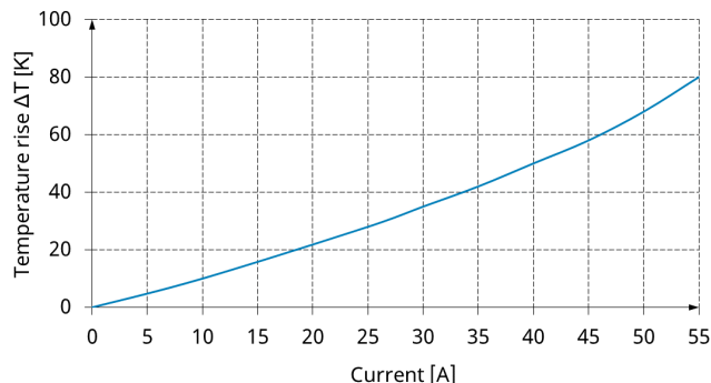
Current Rating
